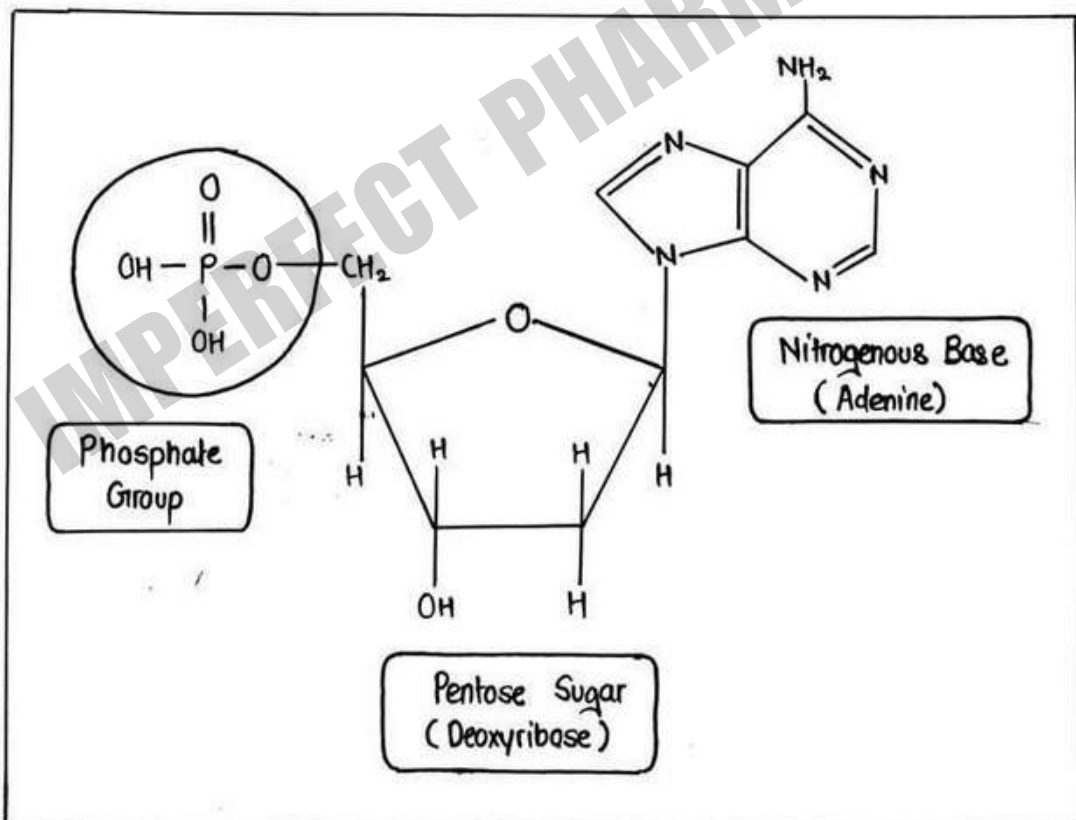
NUCLEOTIDE
