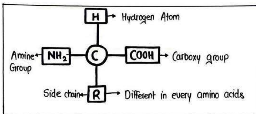
Amino Acid Structure
