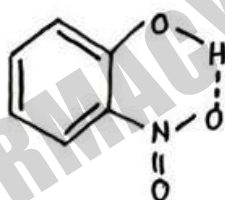
O - Nitrophenol
