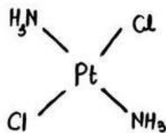
Trans- Platin
