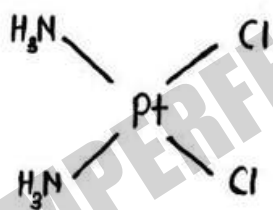
Cis- Platin
