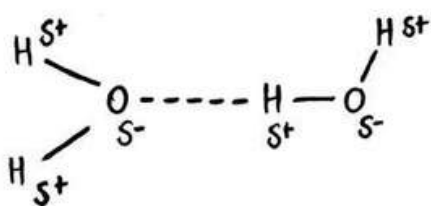
Water
