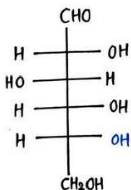
D - Glucose
