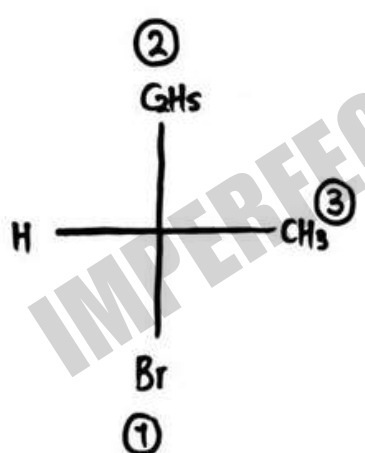
② - 2-Bromobutane
